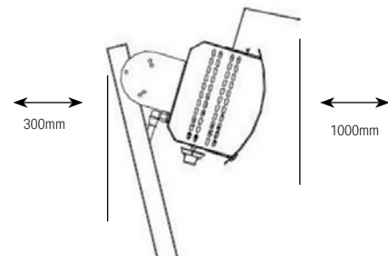
Minimum Clearances from Combustibles (front and rear)
